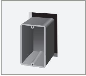
When installing jamb version, cutout dimensions are 1 1/8" (W) x 2 7/8" (H) x 1" (D min)
