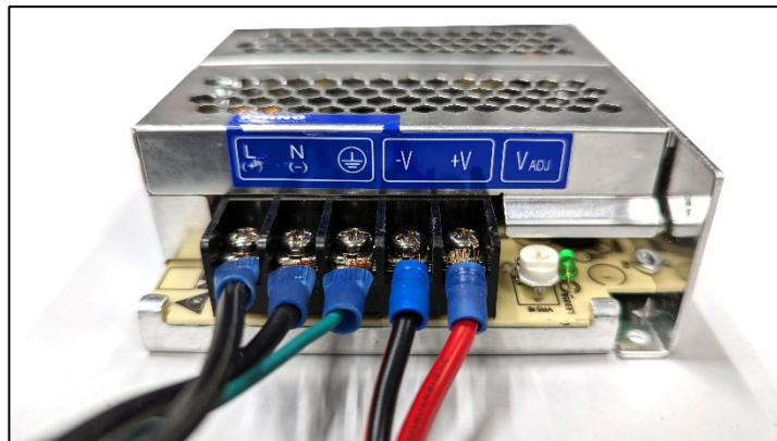
Included Power Supply with Connections
