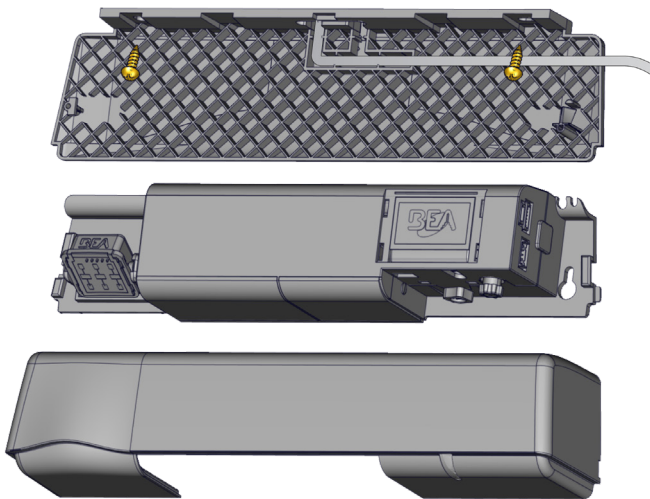
Exploded assembly with ULTIMO sensor
