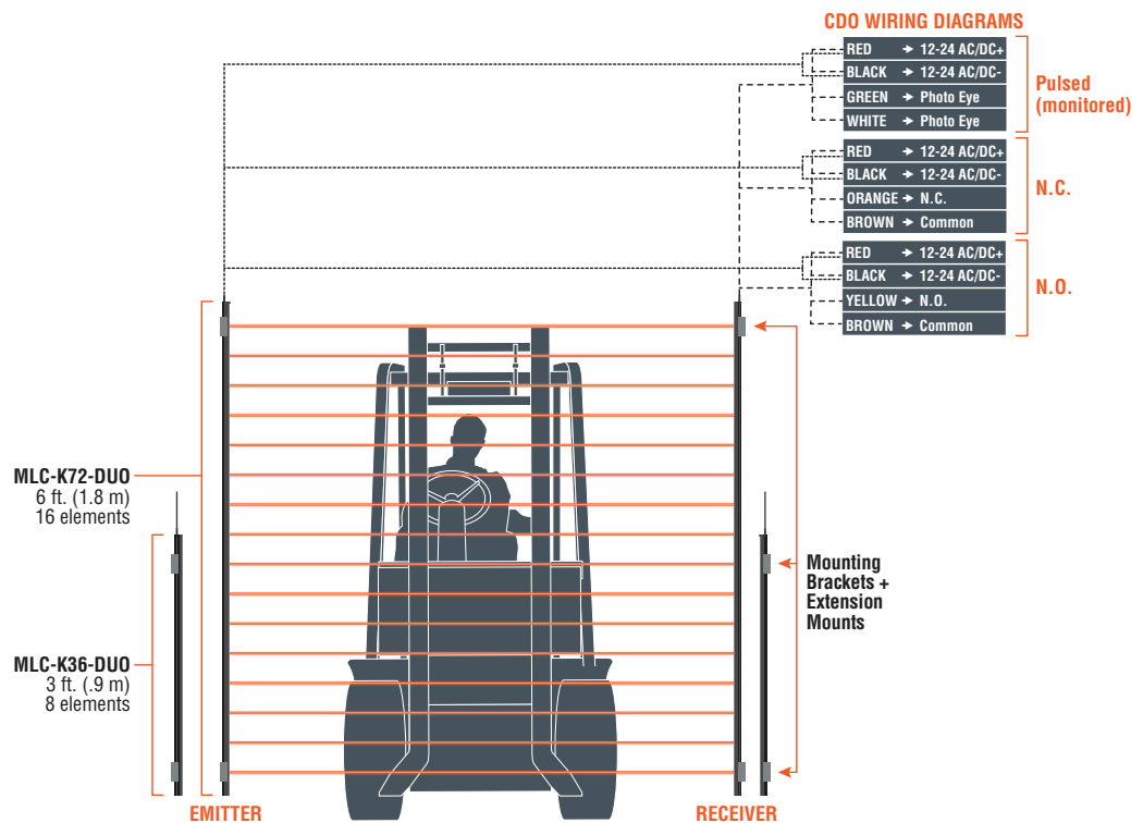
Emitter and receiver units installed showing mounting locations and wiring diagram options
