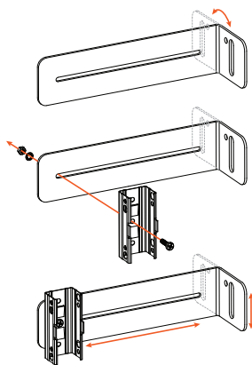
Connecting the universal mounting bracket to the extension mount—height and depth adjustments shown
