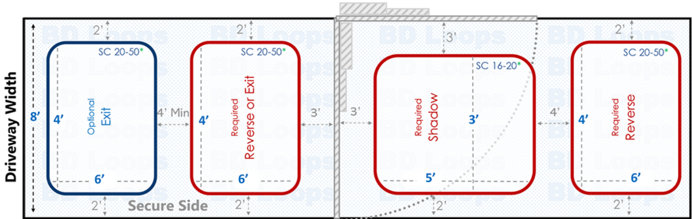
Drawing not to scale.
